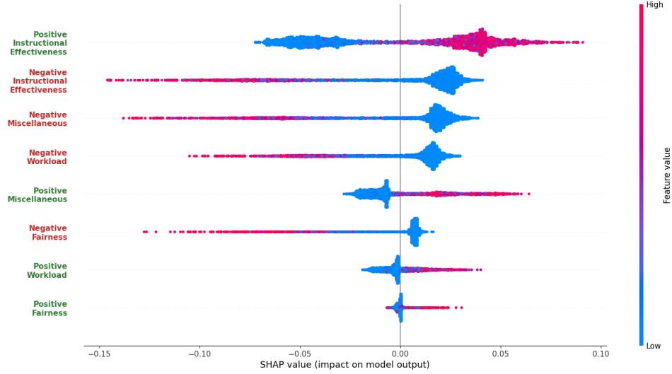
Figure 4. SHAP beeswarm plot for the eight polarity \times topic categories on held-out professors. Point colour indicates feature value; horizontal position shows each feature’s contribution to the predicted rating.
