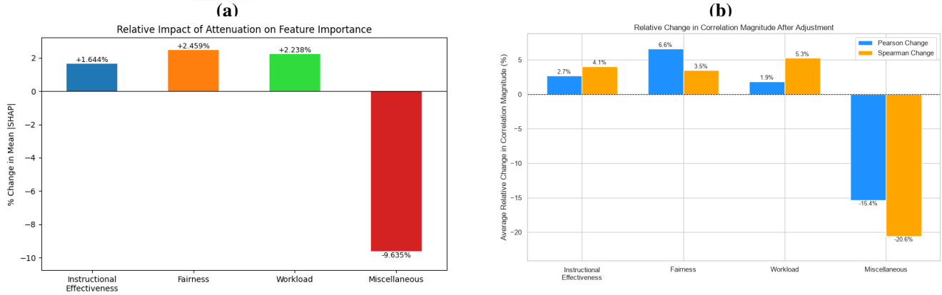
Figure 5. Mechanistic coherence checks after attenuation. (a) Relative changes in SHAP-based feature importance, computed on held-out professors ( n = 3,414 reviews). (b) Average relative change in correlation magnitude (Pearson and Spearman) after adjustment, held-out professors ( n = 2,052 ). Bars show mean (|corr_{adjusted}| - |corr_{raw}|) / |corr_{raw}| across polarity groups.
